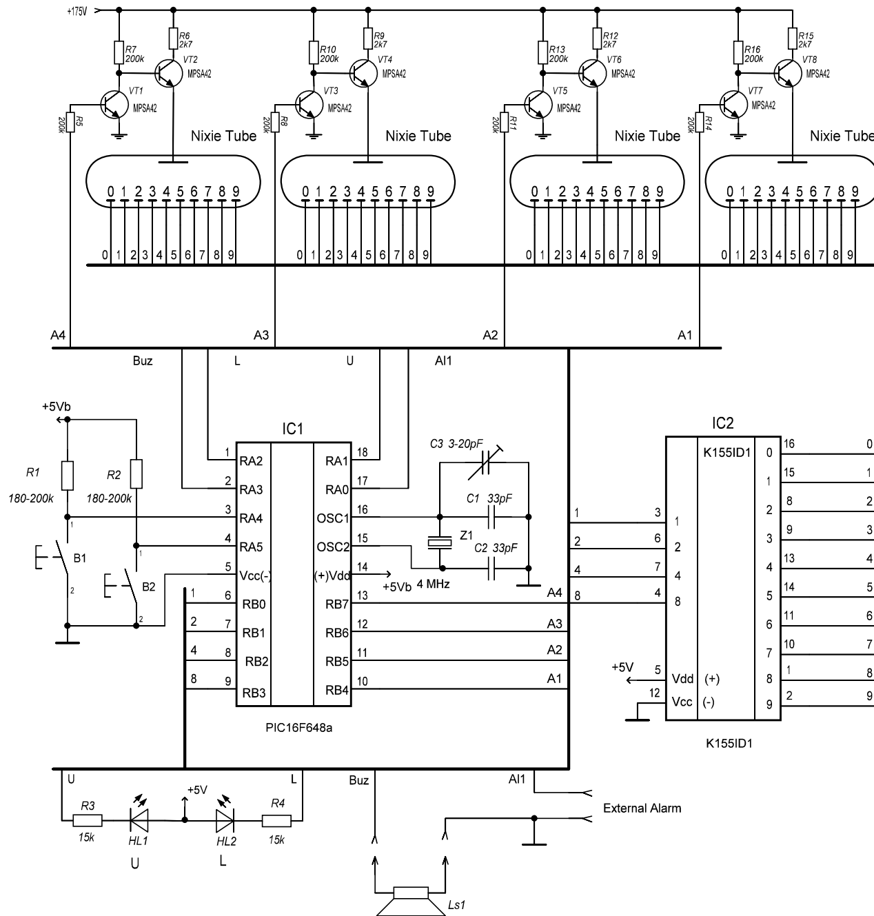
4 digits IN-17 Nixie clock
